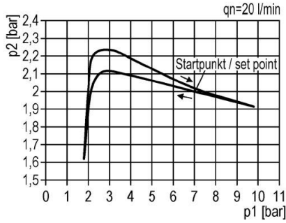
pressure characteristic
